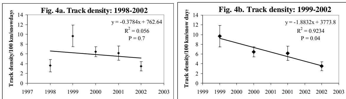
Figure 4. Density of tiger tracks (tracks/100 km/days since last snow) as indicators of tiger abundance on 16 sites included in the Amur Tiger Monitoring Program, a: 1997-1998 through 2001-2002 winters; b: 1998-1999 through 2001-2002 winters.
