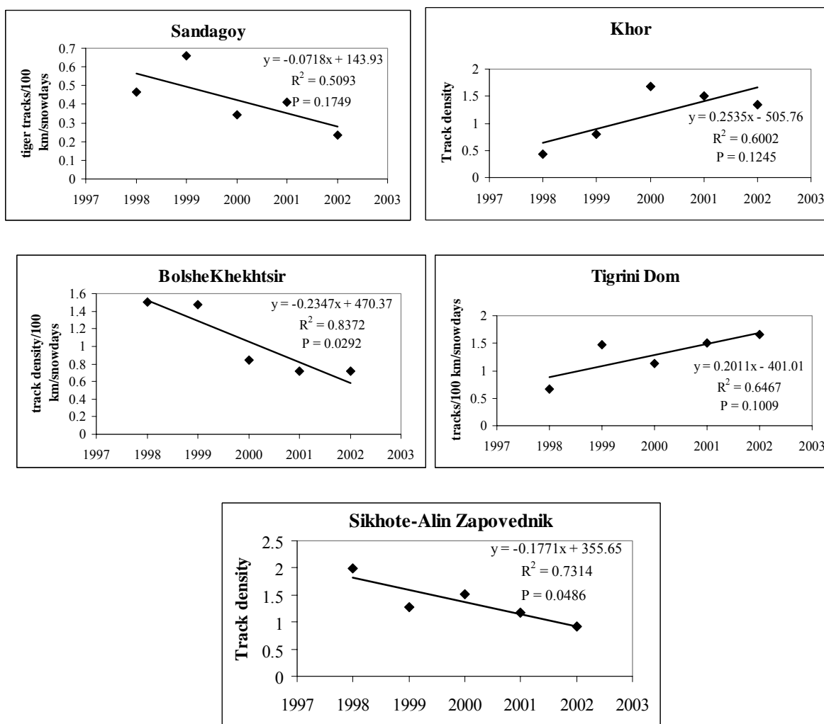
Figures 5a-e. Trends in track density estimators (calculated as the number of tiger tracks/days since last snow x100 km of transects covered) for 5 years on 5 sites for which P-values of the regression analysis (test that B, or slope of the line, does not equal 0) were less than 0.20: a) Sandagoy, b) Khor, c) Bolshe- Khekhtsirski Zapovednik, d) Tigrini Dom, and e) Sikhote-Alin Zapovednik).
